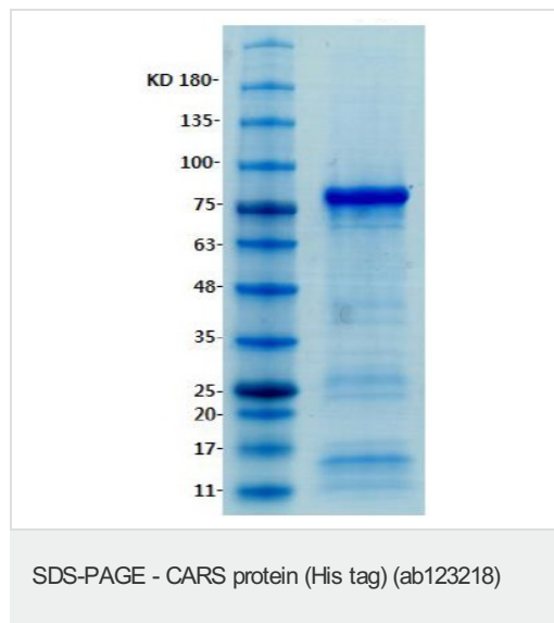
SDS-PAGE analysis of 6ug ab123218 in 4~20% gradient gel
