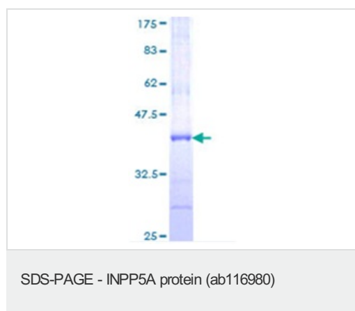
12.5% SDS-PAGE Stained with Coomassie Blue.
