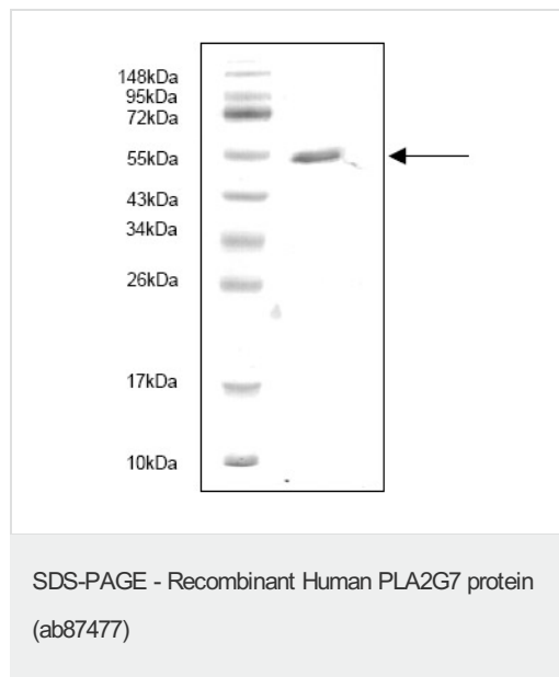
ab87477 on SDS-PAGE.
