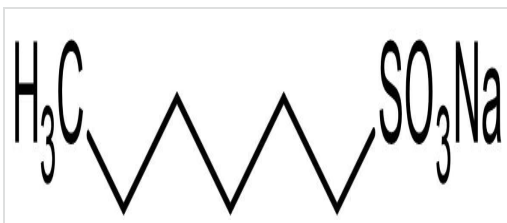
Chemical Structure - 1-Hexanesulfonic acid sodium salt, Anionic surfactant (ab146209)
