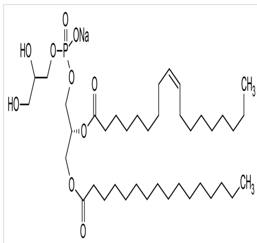
Chemical Structure - 1-Palmitoyl-2-oleoyl-sn-glycero-3-phosphorylglycerol sodium salt, Phosphatidylglycerol component (ab143959)
