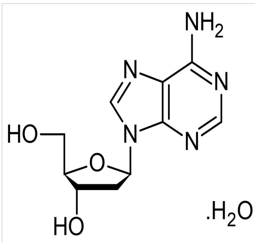
Chemical Structure - 2'-Deoxyadenosine monohydrate, deoxyribonucleoside (ab146527)
