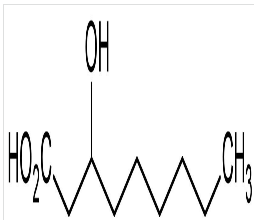
Chemical Structure - 3-Hydroxynonanoic acid, Nonesterified 3-hydroxy fatty acid (ab144024)
