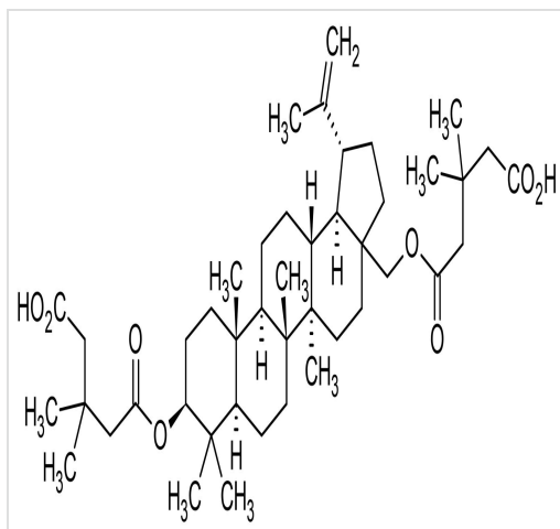
Chemical Structure - 3,28-Di-O-(3,3-dimethylglutaryl)betulin, Semisynthetic derivative of betulin (ab144242)
