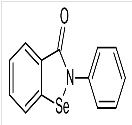
Chemical Structure - Ebselen, mimic of glutathione peroxidase (ab142424)
