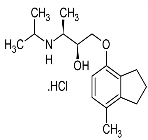
2D chemical structure image of ab120808, ICI 118551 hydrochloride, beta2 adrenoceptor antagonist
