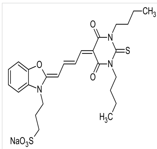
2D chemical structure image of ab145391, Merocyanin 540 (Merocyanine 540), Fluorescent membrane indicator
