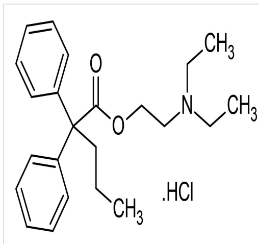
2D chemical structure image of ab144624, Proadifen hydrochloride (SKF-525A), Cytochrome P450 inhibitor
