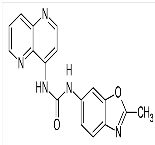
Chemical Structure - SB 334867, OX 1 receptor antagonist (ab120164)
