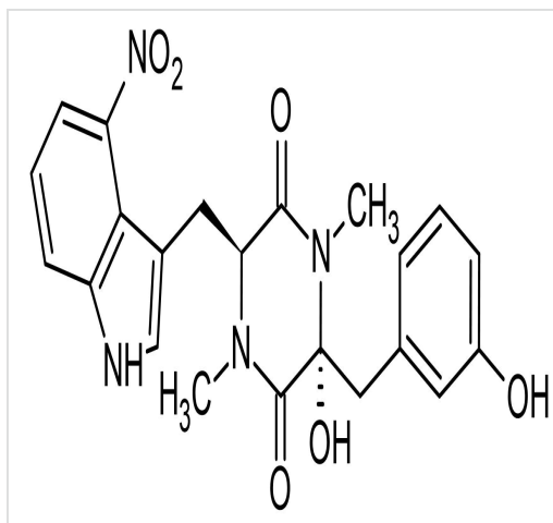
Chemical Structure - Thaxtomin A, Cellulose synthesis inhibitor (ab144372)
