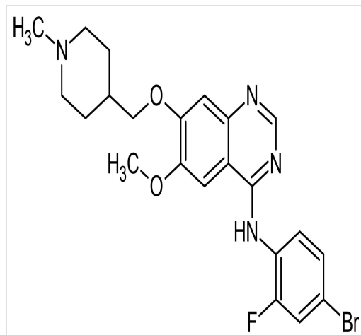
Chemical Structure - Vandetanib, VEGFR2 tyrosine kinase inhibitor (ab142099)
