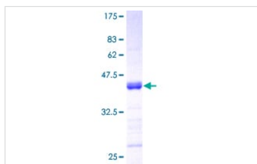
ab160170 on a 12.5% SDS-PAGE stained with Coomassie Blue.
