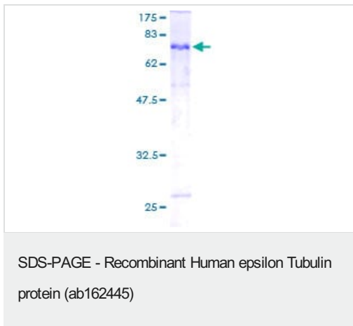
ab162445 on a 12.5% SDS-PAGE stained with Coomassie Blue.
