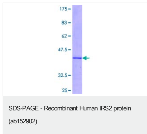
ab152902 on a 12.5% SDS-PAGE stained with Coomassie Blue.
