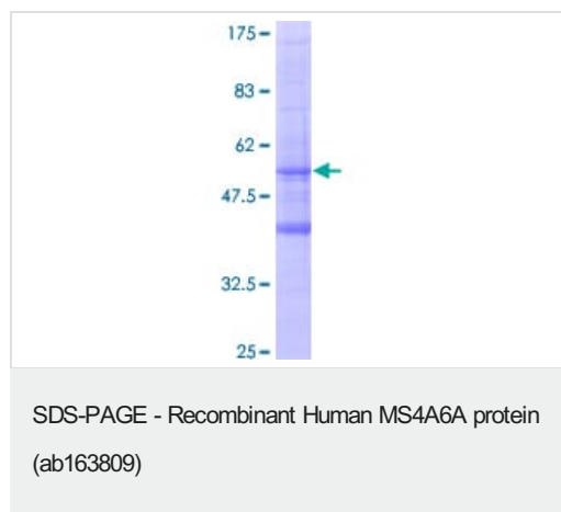
ab163809 on a 12.5% SDS-PAGE stained with Coomassie Blue.
