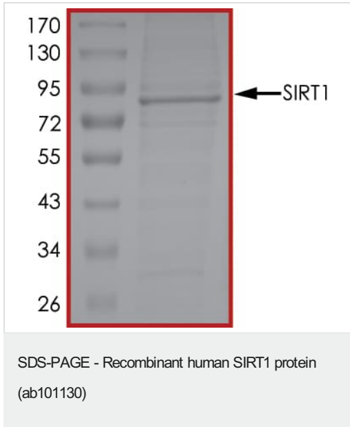
SDS PAGE analysis of ab101130
