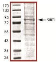
SDS-PAGE - Recombinant human SIRT1 protein (ab101130)
