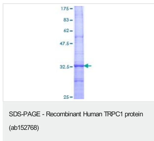
12.5% SDS-PAGE analysis of ab152768 stained with Coomassie Blue.
