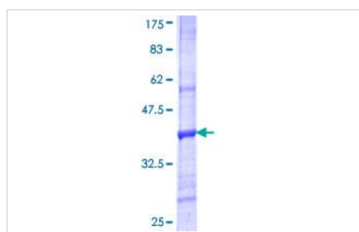
ab163077 on a 12.5% SDS-PAGE stained with Coomassie Blue.
