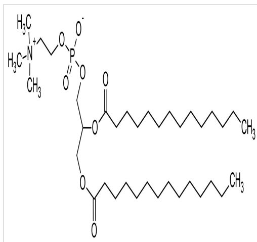
Chemical Structure - 1,2-Dimyristoyl-sn-glycero-3-phosphorylcholine (DMPC), Phosphatidylcholine (ab143946)
