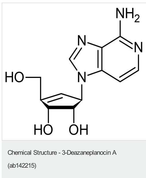
2D chemical structure image of ab142215, 3-Deazaneplanocin A
