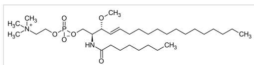
Chemical Structure - 3-O-Methyl-sphingomyelin, neutral sphingomyelinase inhibitor (ab141756)
