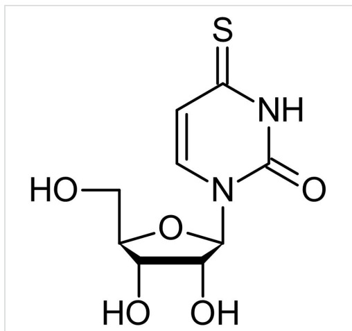
Chemical Structure - 4-Thiouridine, RNA synthesis inhibitor (ab143718)
