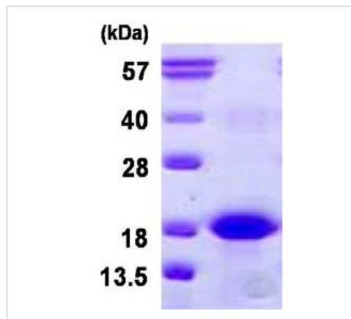
15% SDS-PAGE showing ab126683 (3 µg)
