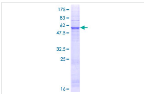
ab166154 on a 12.5% SDS-PAGE stained with Coomassie Blue.
