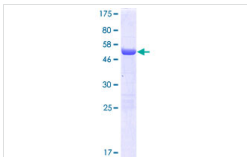
ab166224 on a 12.5% SDS-PAGE stained with Coomassie Blue.
