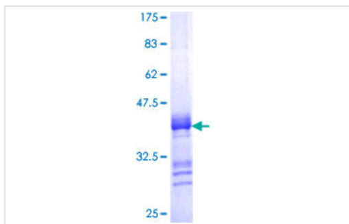
ab165050 on a 12.5% SDS-PAGE stained with Coomassie Blue.
