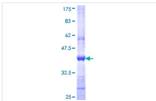
SDS-PAGE - Recombinant Human PIB5PA protein (ab162085)
