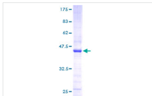
ab159224 on a 12.5% SDS-PAGE stained with Coomassie Blue.
