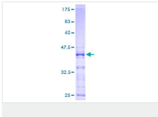
ab159458 on a 12.5% SDS-PAGE stained with Coomassie Blue.
