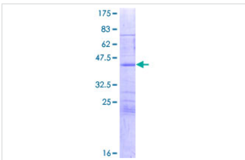
SDS-PAGE - Recombinant Human Spir-1 protein (ab163422)
