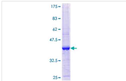
ab161687 on a 12.5% SDS-PAGE stained with Coomassie Blue.
