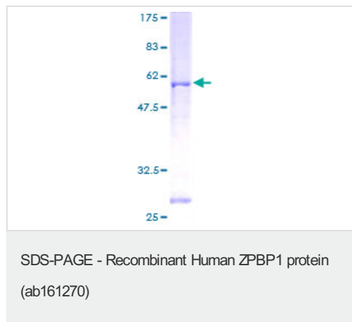
ab161270 on a 12.5% SDS-PAGE stained with Coomassie Blue.
