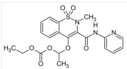
Chemical Structure - Ampiroxicam, cyclooxygenase inhibitor (ab142826)
