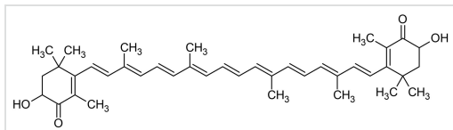
Chemical Structure - Astaxanthin, Antioxidant agent (ab144193)
