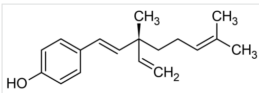
Chemical Structure - Bakuchiol, Resveratrol analog (ab141036)
