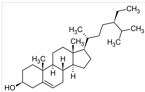
Chemical Structure - beta-Sitosterol, Antitumor agent (ab143122)
