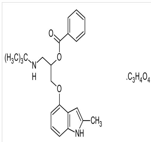
Chemical Structure - Bopindolol malonate, adrenoceptor antagonist (ab141516)
