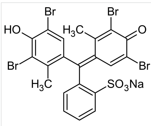
Chemical Structure - Bromocresol green sodium salt, electrophoresis tracking dye (ab146289)
