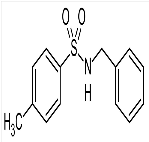
Chemical Structure - BTS, Ca 2+ -stimulated myosin S1 ATPase (ab145875)
