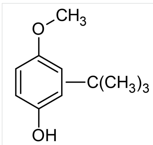
Chemical Structure - Butylated hydroxyanisole (BHA), Phenolic anti-oxidant (ab142841)
