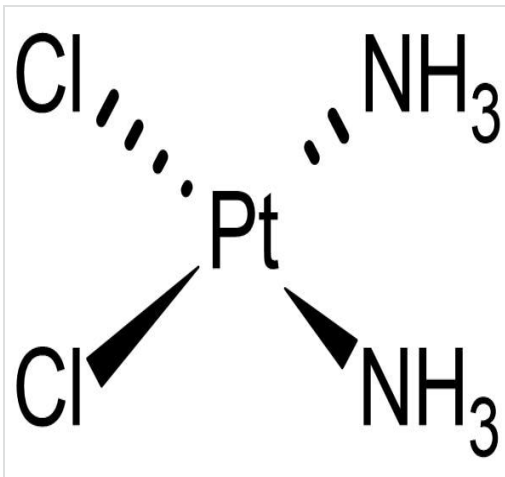
Chemical Structure - Cisplatin, antineoplastic agent (ab141398)
