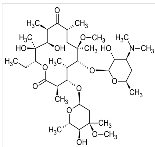
Chemical Structure - Clarithromycin, Macrolide antibiotic (ab141202)
