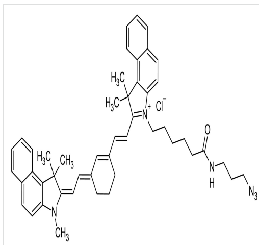
Chemical Structure - Cyanine7.5 azide, NIR emitting fluorescent dye azide (ab146475)
