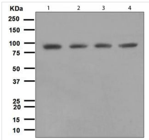
Western blot - Anti-DDX50 antibody [EPR5273] (ab109515)
