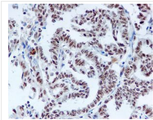
Immunohistochemistry (Formalin/PFA-fixed paraffin-embedded sections) - Anti-DDX50 antibody [EPR5273] (ab109515)
