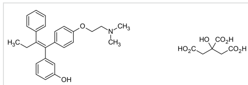
2D chemical structure image of ab142745, Droloxifene citrate, estrogen receptor antagonist
