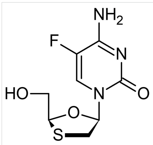
Chemical Structure - Emtricitabine, reverse transcriptase inhibitor (ab145045)
